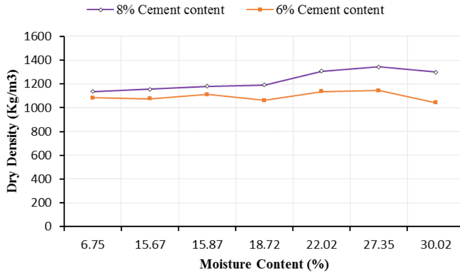
Figure 2: Variation of DD with MC at 15% RHA
