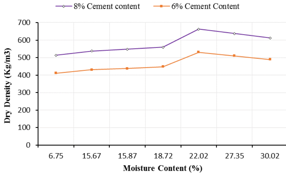
Figure 1: Variation of DD with MC at 0% RHA
