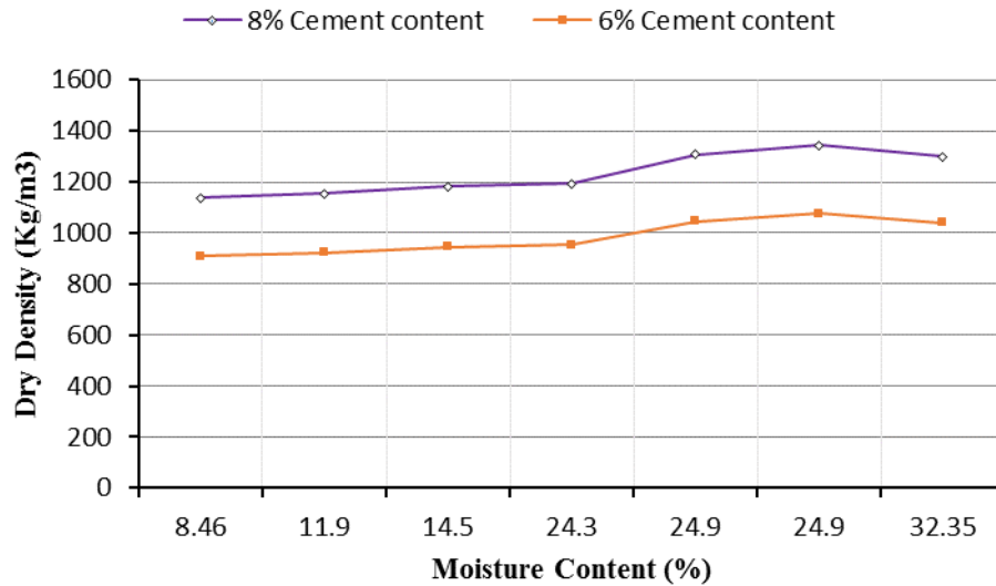
Figure 4: Variation of DD with MC at 45% RHA
