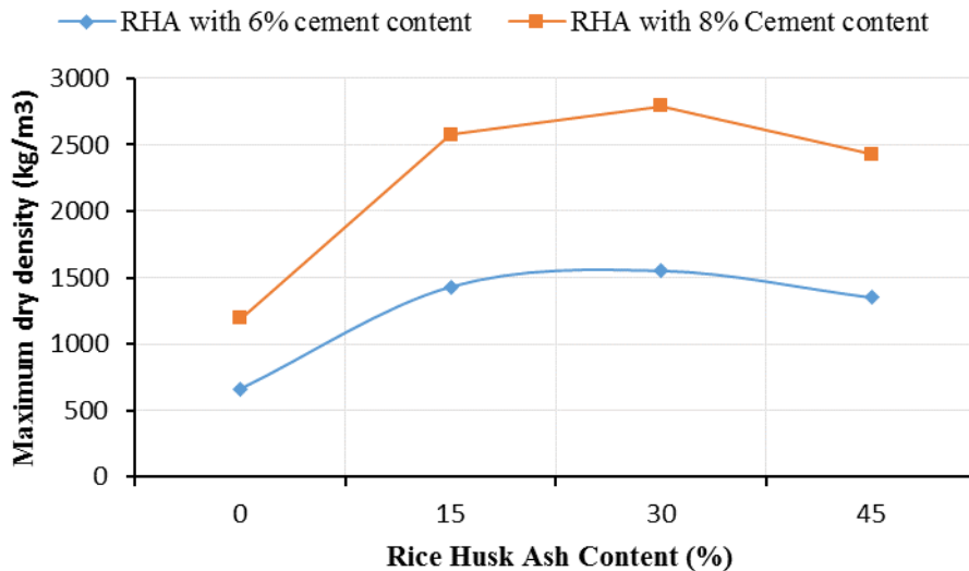
Figure 5: Variation of MDD with RHA-Cement Blend
