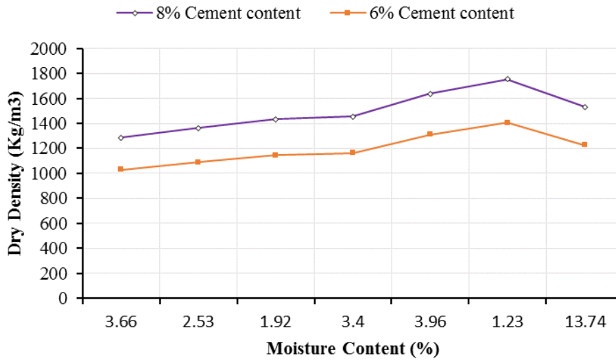
Figure 3: Variation of DD with MC at 30% RHA
