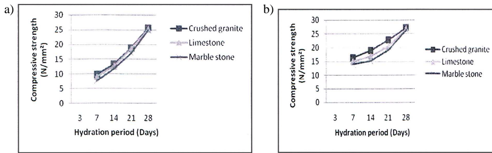
Fig. 2. Compressive strength of the concrete produced from the various coarse aggregate at water cement ratios of (a) 0.5 and (b) 0.06, and design concrete strengths of 30 N/mm 2
