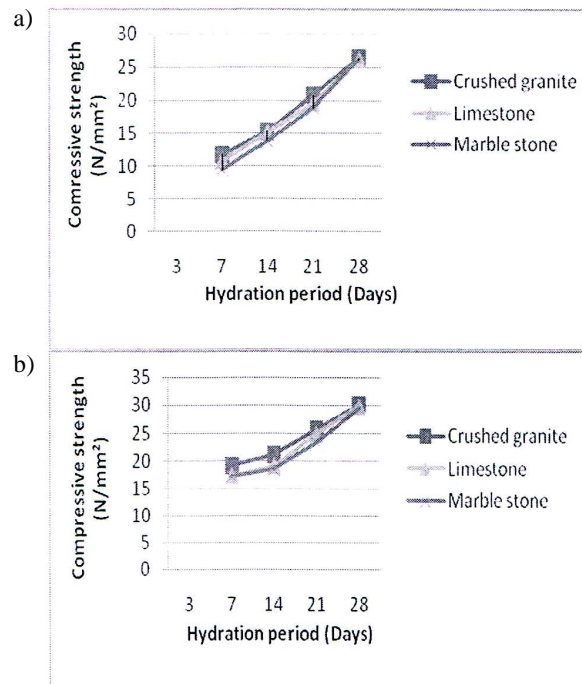
Fig. 1. Compressive strength of the concrete produced from the various coarse at water cement ratios of: a) 0.5 and b) 0.6, and design concrete strengths of 20 N/mm 2
